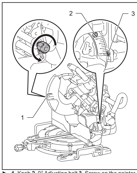
► 1. Knob 2. 0° Adjusting bolt 3. Screw on the pointer
