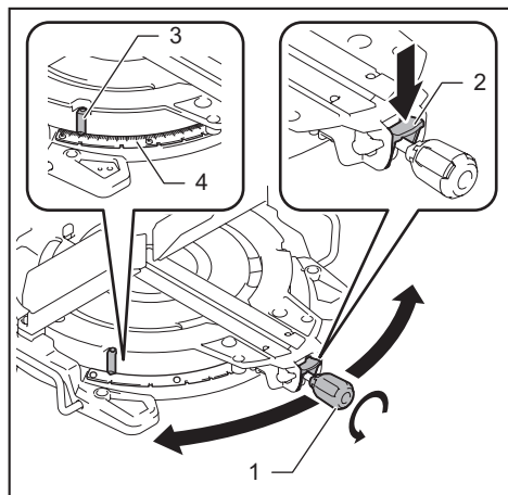
► 1. Grip 2. Lock lever 3. Pointer 4. Miter angle scale
