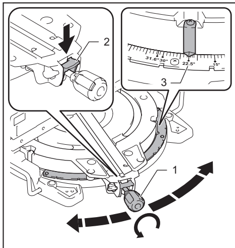
► 1. Grip 2. Lock lever 3. Positive stop angle
