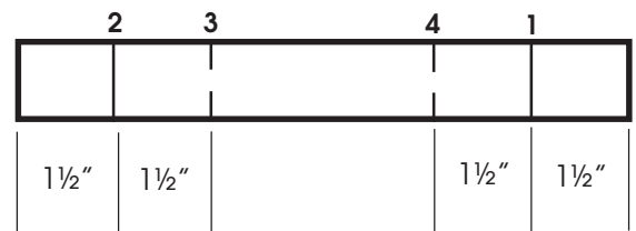
Bend Sequence
