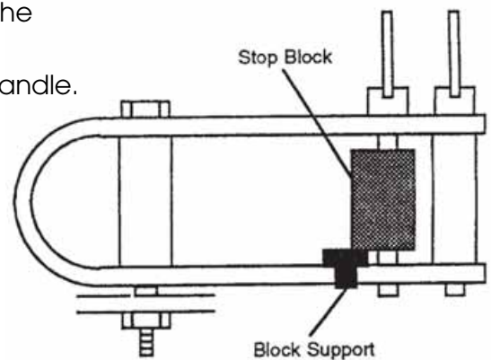
Positioning the Block Support
